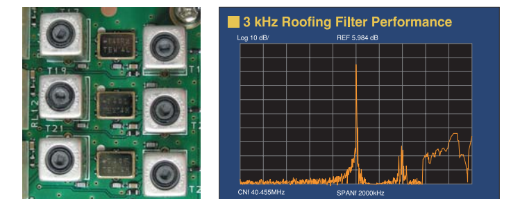
Three Selections of IF Roofing Filters 10 dB/Div · 200 kHz/Div
